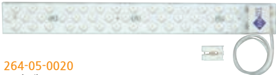
264-05-0020 포밍 램프 20W Size W405XH48 Lamp LED 20W / 6500K
