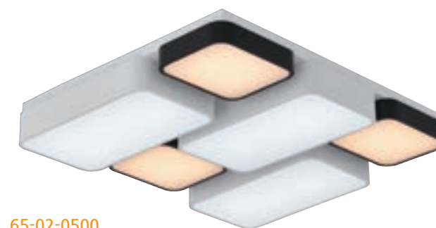
65-02-0500 믹스거실 6등 Size W845XD720XH100 Lamp LED 180W Color 화이트+블랙
